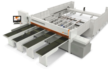
AXO 500 T HD Asansörlü Panel Ebatlama Makinesi Automatic Panel Saws With Lifting Table
